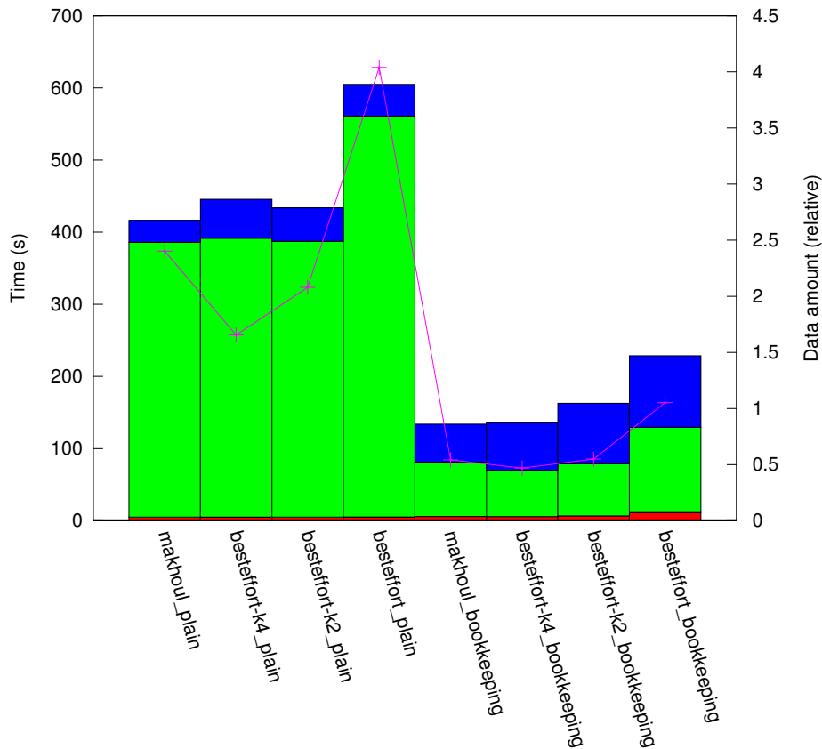
results_IN_1:10/plat_grid64/topo_torus
