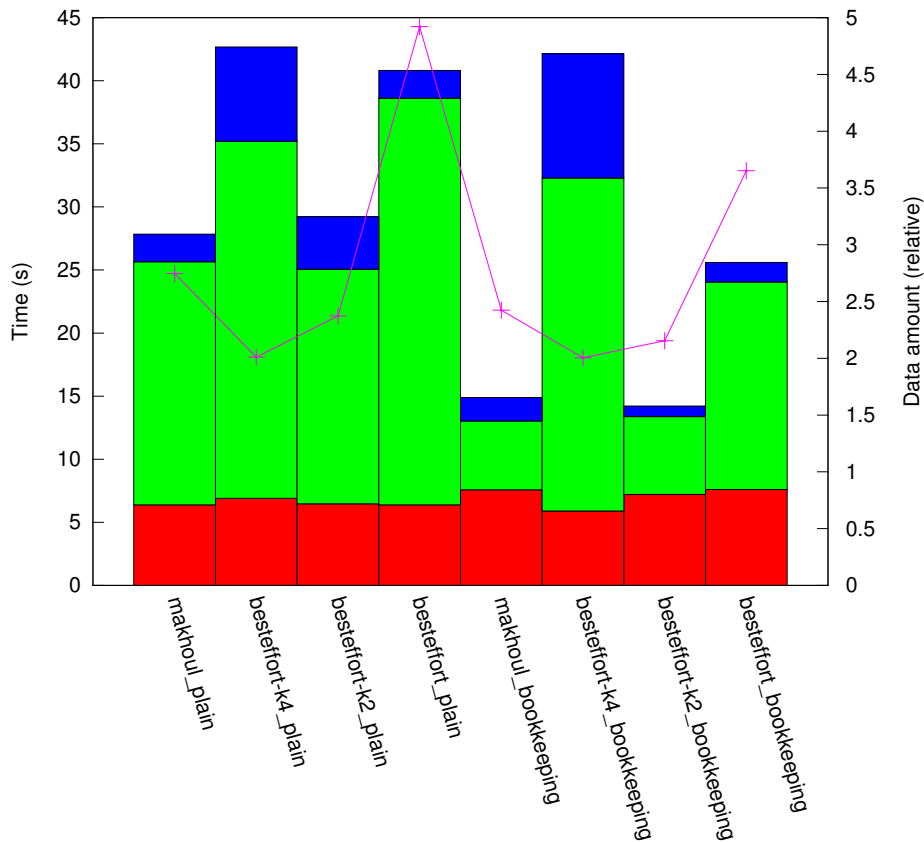
results_I1_10:1/plat_cluster16/topo_hcube
