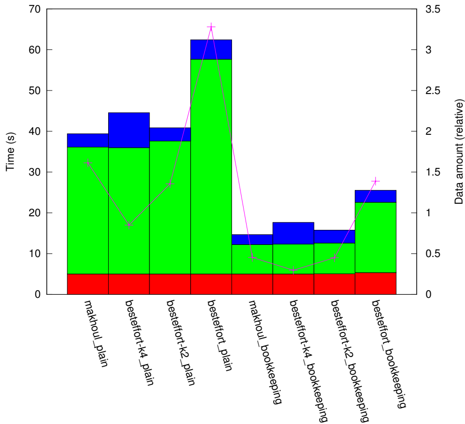
results_IN_1:1/plat_cluster16/topo_torus
