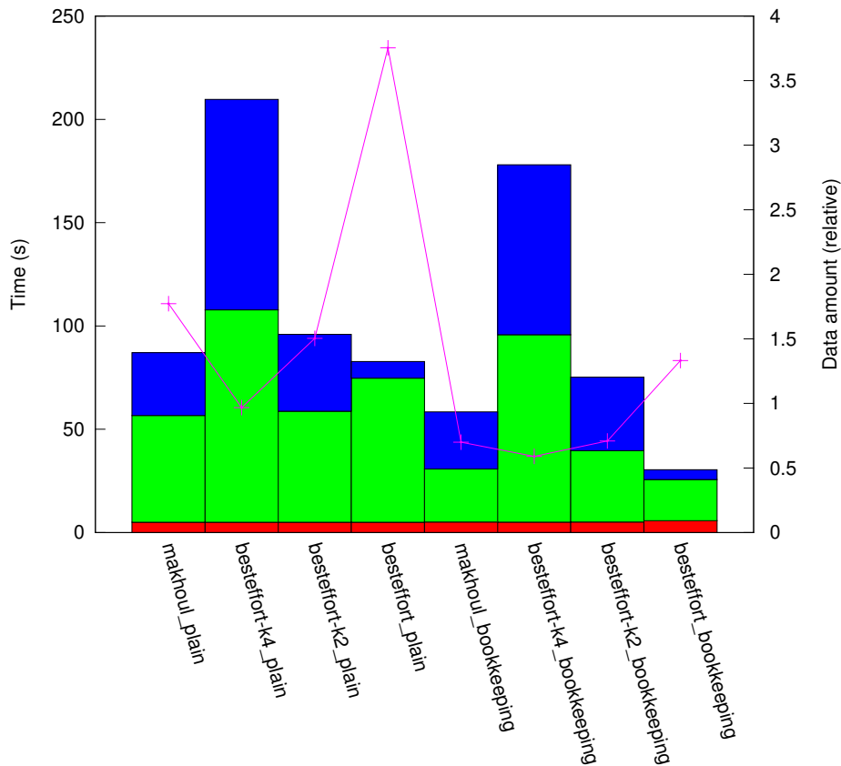
results_IN_1:1/plat_cluster256/topo_torus
