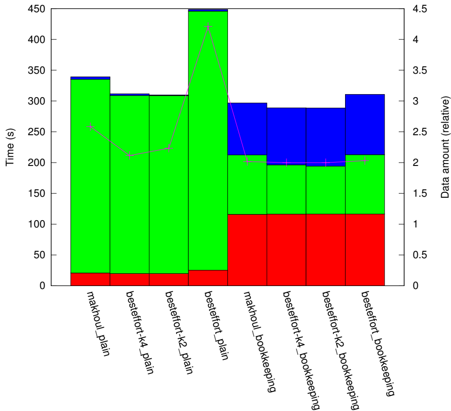
results_l1_1:10/plat_cluster16/topo_torus
