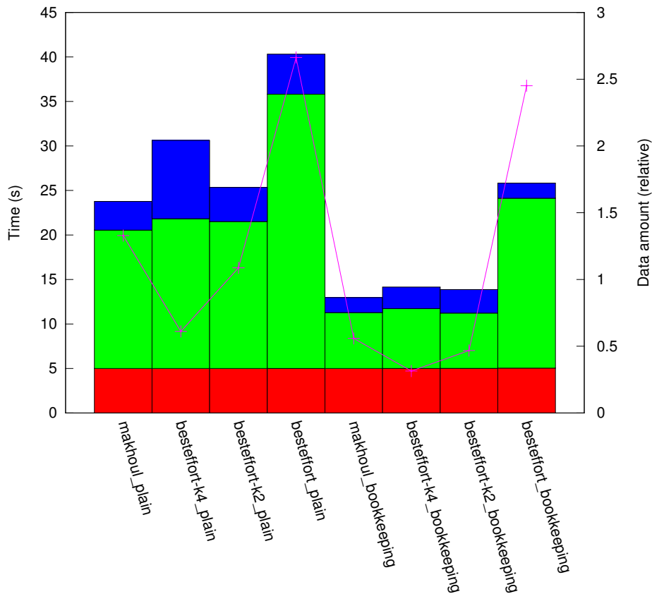
results_IN_10:1/plat_cluster16/topo_hcube
