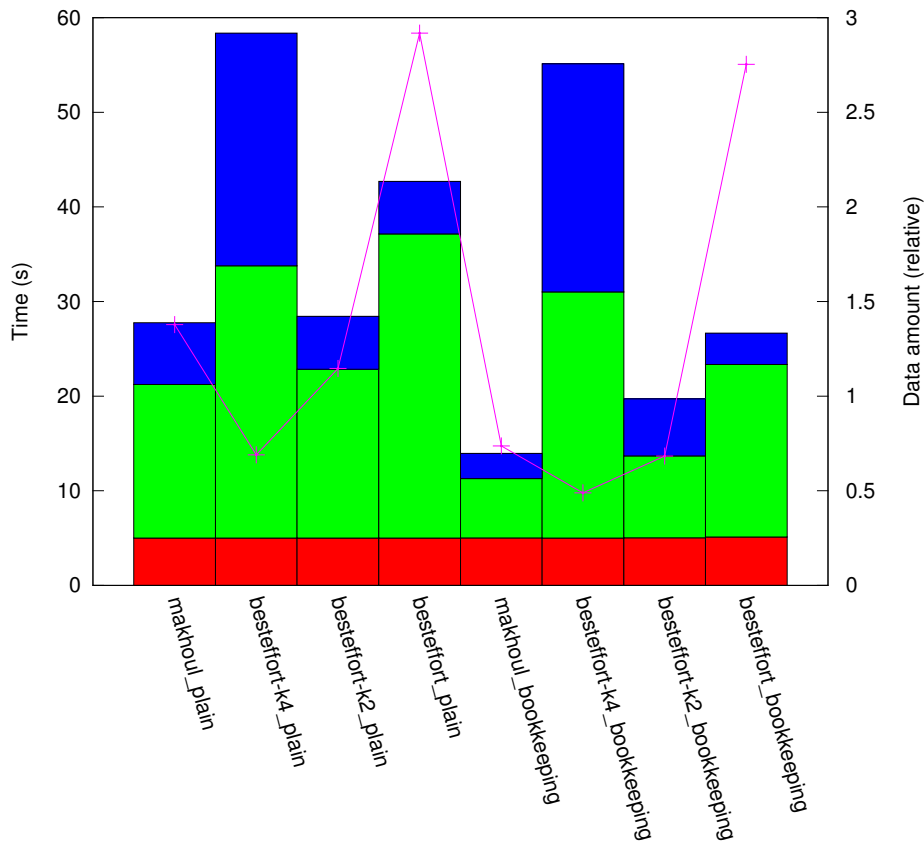
results_IN_10:1/plat_cluster64/topo_torus
