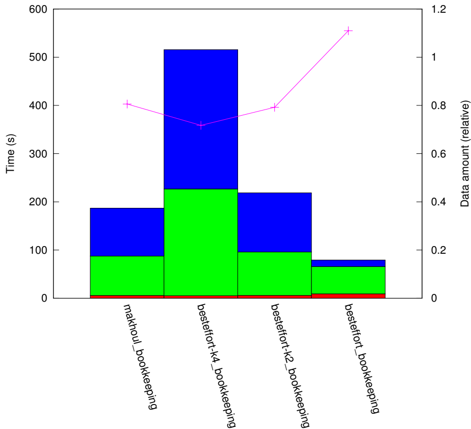
results_IN_1:1/plat_cluster1024/topo_torus
