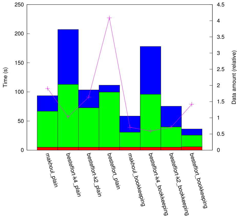
results_IN_1:1/plat_grid256/topo_torus
