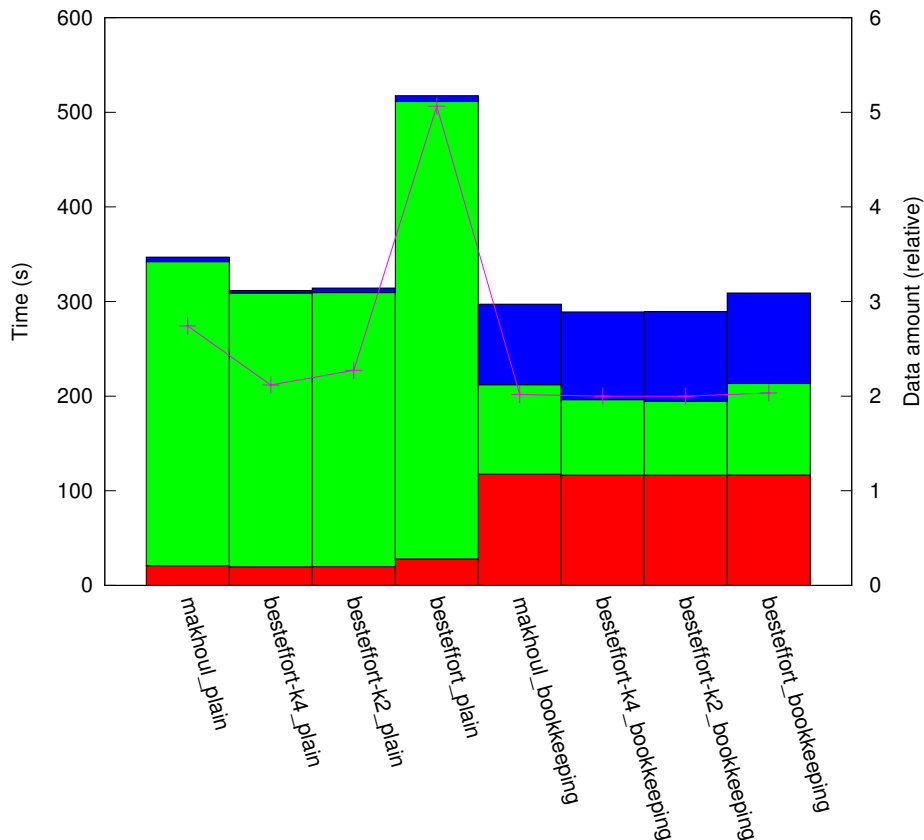
results_R1_1:10/plat_cluster16/topo_hcube
