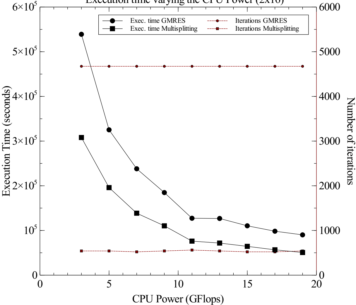
Execution time varying the CPU Power (2x16)
