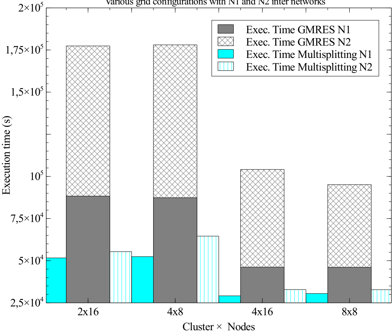
Various grid configurations with N1 and N2 inter networks
