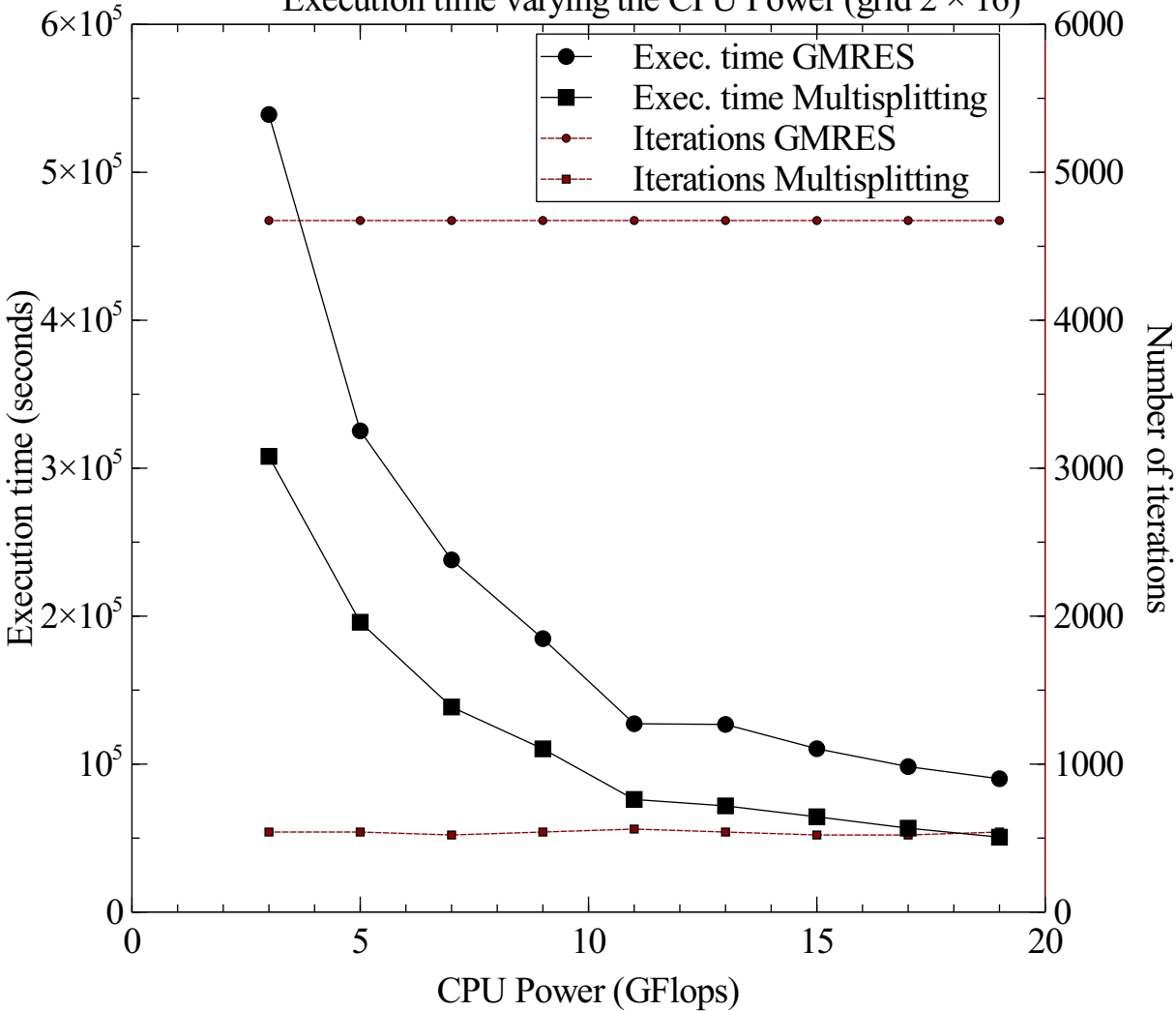
Execution time varying the CPU Power (grid 2 \times 16 )
