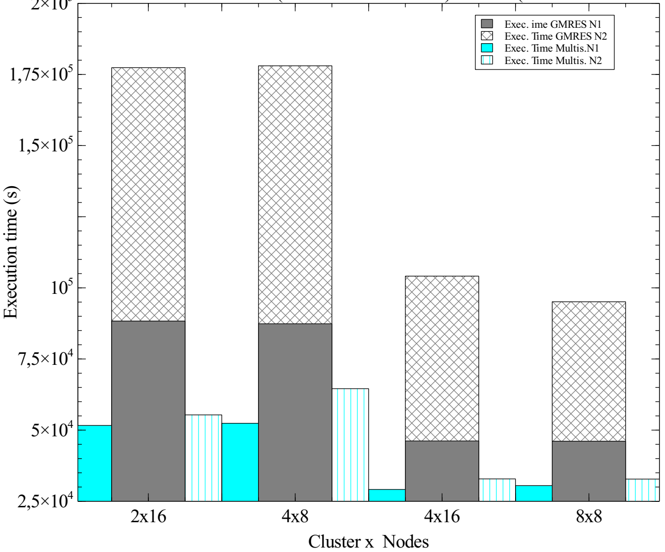
2 Clusters x 16 Nodes N1 (bw=10Gbit/s-lat=8E-6) and N2 (bw=1Gbit/s-lat=5E-5)
