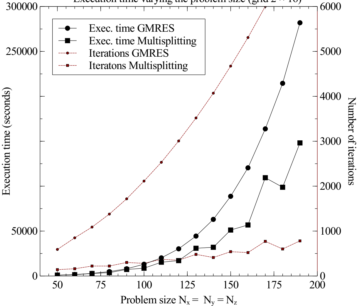
Execution time varying the problem size (grid 2 \times 16 )
