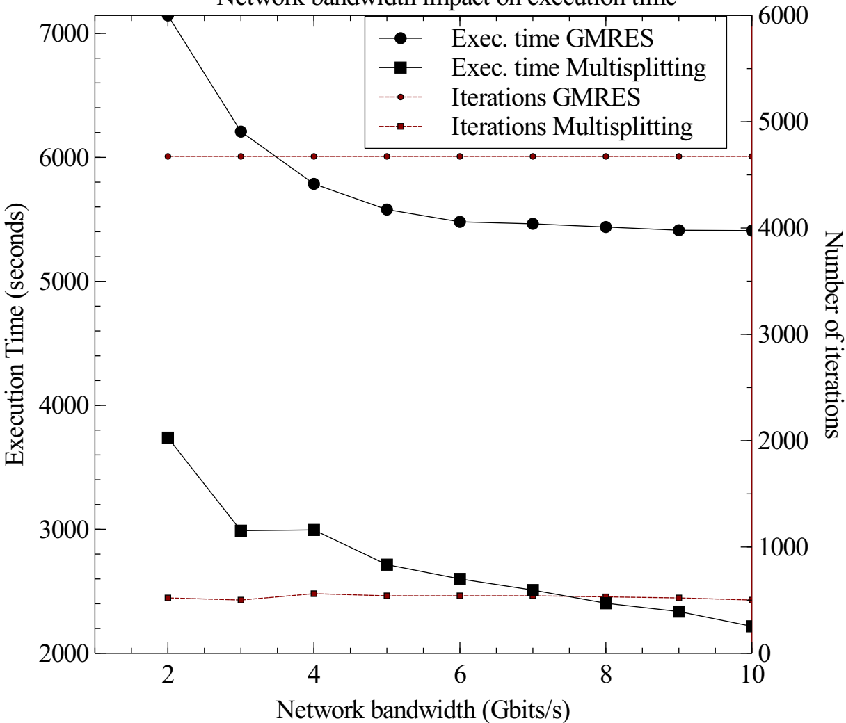
Network bandwidth impact on execution time
