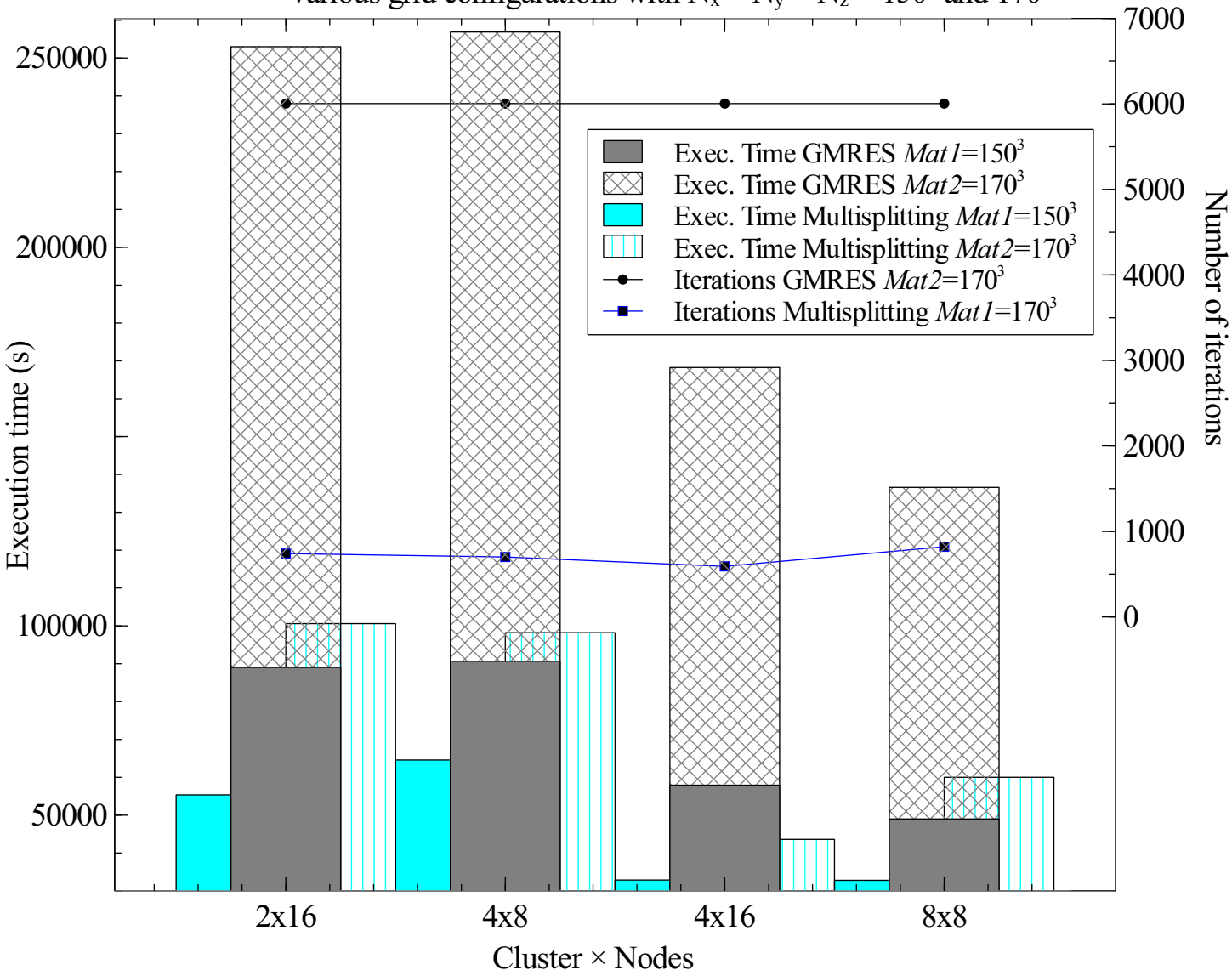
Various grid configurations with N_x \times N_y \times N_z = 150^3 and 170^3
