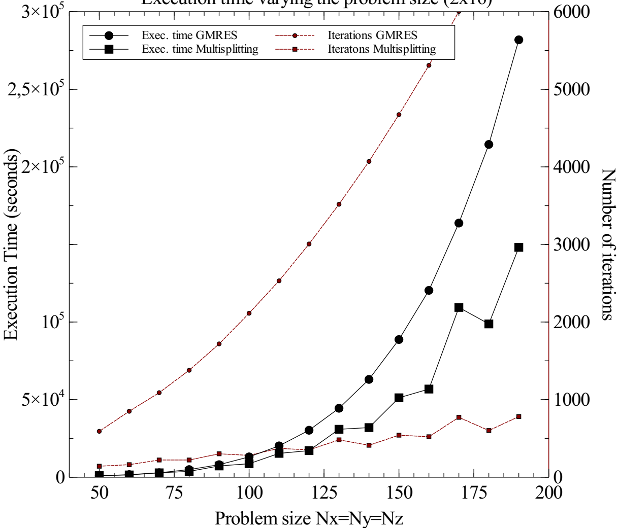
Execution time varying the problem size (2x16)
