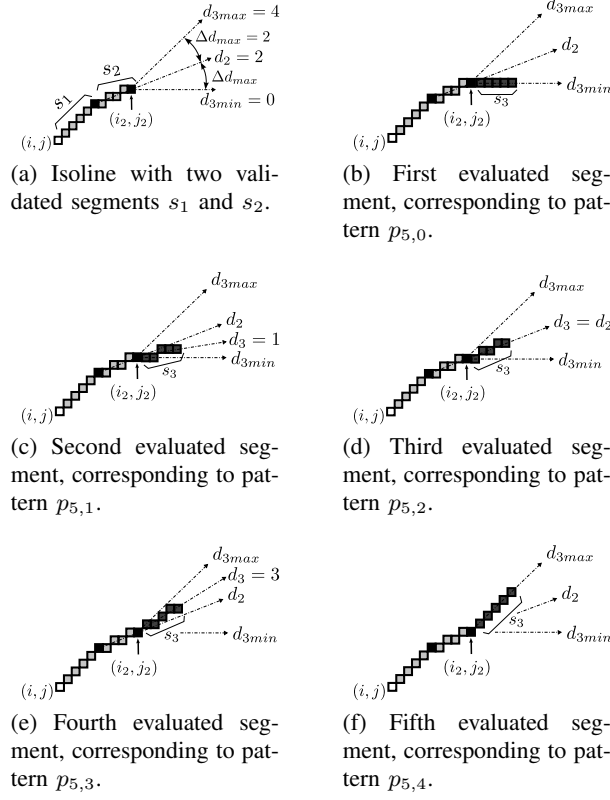
Fig. 2. Example of lengthening process starting with a two-segment poly-isoline ( l = 5 , \Delta d_{max} = 2 ). The initial situation is shown in 2a, while 2b to 2f represent the successive candidate segments. The direction index of the last validated segment is d_2 = 2 (2a). It implies that direction indexes allowed for the third segment range from d_2 - \Delta d_{max} = 0 to d_2 + \Delta d_{max} = 4 (2b to 2f). The lengthening of the poly-isoline is accepted if at least one segment has a positive GLRT. If there are several, the one which minimizes the standard deviation of the whole poly-isoline is selected.
