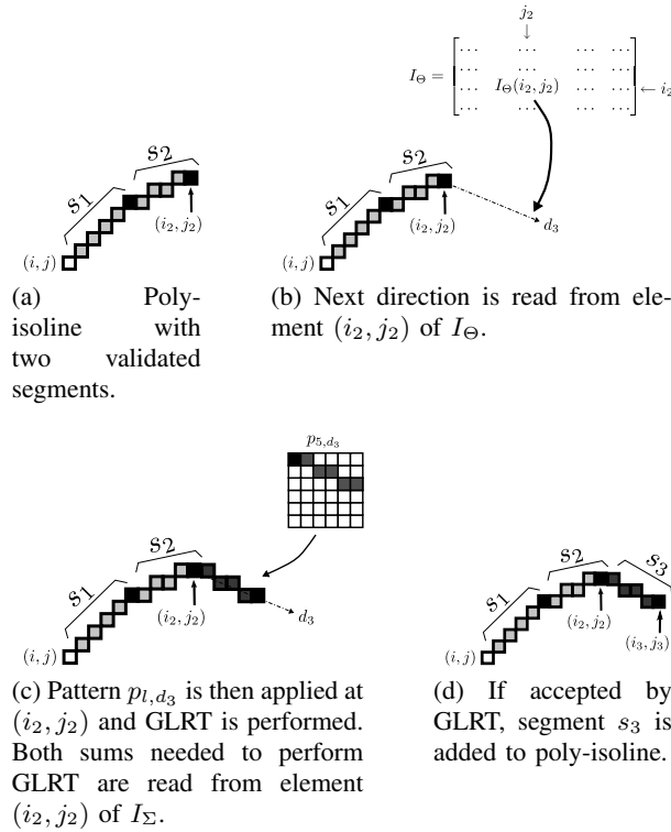
Fig. 3. Example of PI-PD lengthening process starting with a two-segment poly-isoline ( l = 5 ). The initial situation is represented in 3a, while 3a to 3d represent the successive processing steps. The end pixel of the last validated segment is (i_2, j_2) (3a). Reference matrices I_\Theta and I_\Sigma provide the values needed to select the pattern to be applied on (i_2, j_2) (3b and 3c). GLRT is performed to validated lengthening or not. This process goes on until one submitted segment does not comply with GLRT.
