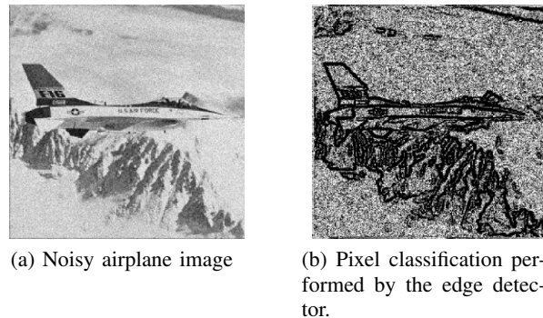
Fig. 7. Pixel classification inside the noisy image. Figure 7a shows the noisy input image and 7b reproduces the output classification of pixels, as a black and white image, obtained with threshold value T_{2max} = 2 . Black pixels are supposed to be near an edge, while white pixels belong to Low Slope Regions.
