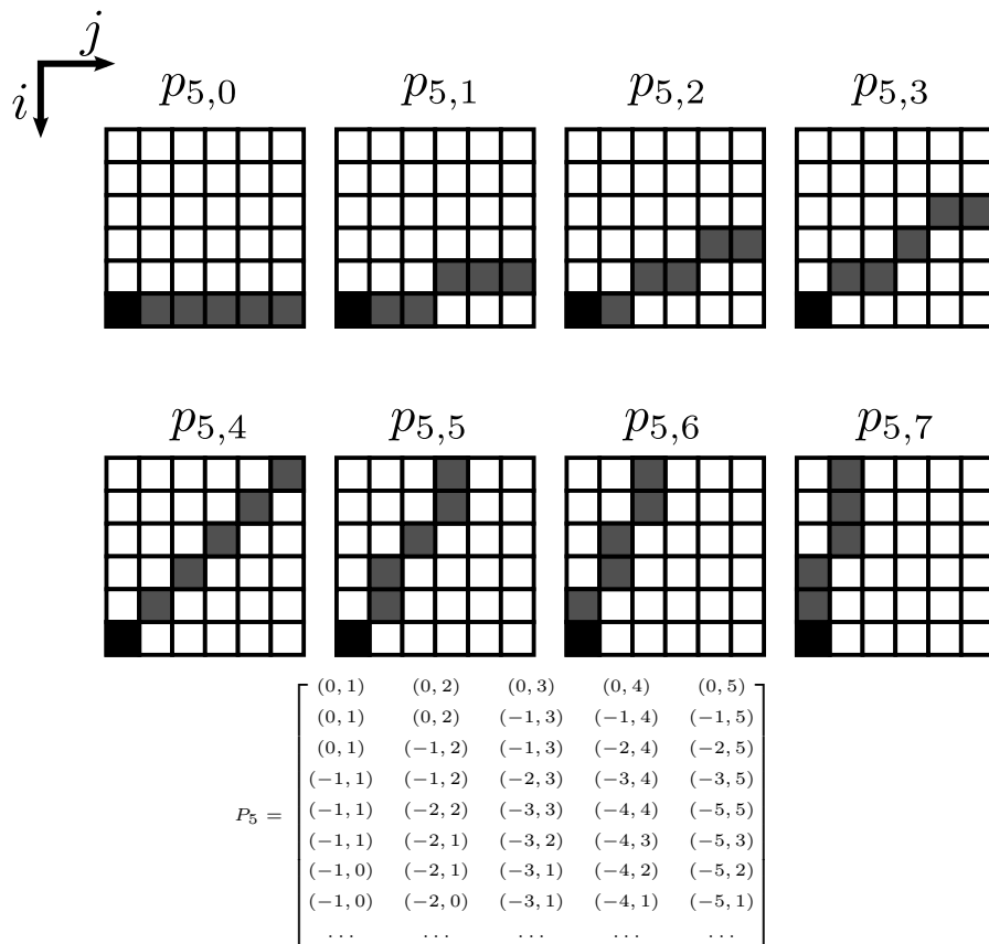
Fig. 8. Top: example segment patterns p_{5,d} for d \in [0;7] ; the black pixel represents the center pixel (i, j) , which does not belong to the pattern. The gray ones define the actual pattern segments. Bottom: the first 8 lines of corresponding matrix P_5 whose elements are the positions of segment pixels with respect to the center pixel.
