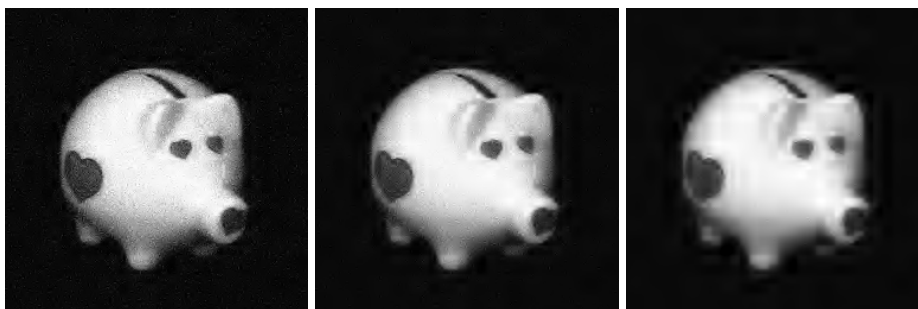
(a) T = 20 , PSNR=26.9 dB, MSSIM=0.30 (b) T = 35 , PSNR=27.6 dB, MSSIM=0.36 (c) T = 70 , PSNR=26.7 dB, MSSIM=0.37
