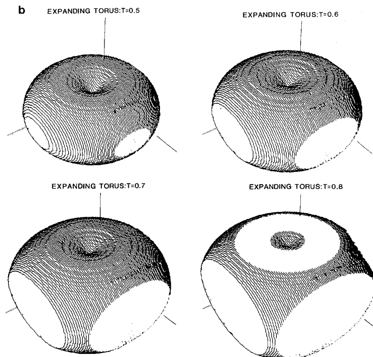
FIG. 12b. Burning torus: change of topology (Continued): F(K) = 1 - \varepsilon K , \varepsilon = 0.01 , surface at T = 0.5, 0.6, 0.7, 0.8 .
