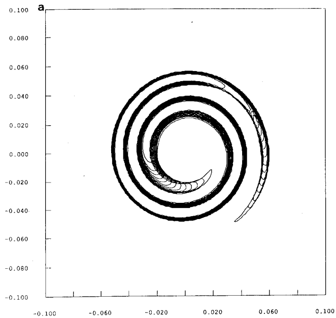
FIG. 5a. Wound spiral collapsing under curvature (Beginning): F(K) = -K , T = 0.0, 0.065 (0.005).
