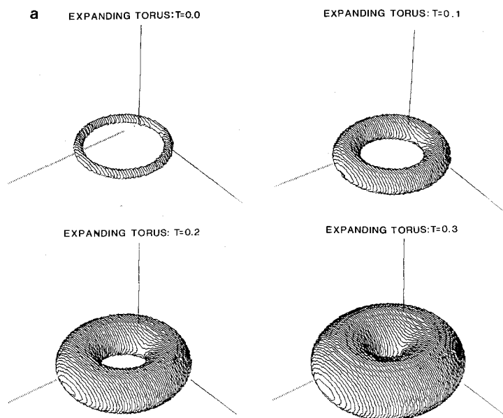
FIG. 12a. Burning Torus: Change of Topology (Beginning): F(K) = 1 - \varepsilon K , \varepsilon = 0.01 , surface at T = 0.0, 0.1, 0.2, 0.3 .
