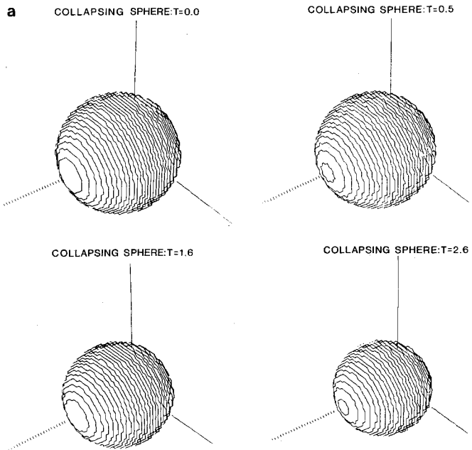
FIG. 13a. Sphere collapsing under mean curvature (Beginning): F(K) = -K , surface at T = 0.0, 0.5, 1.6, 2.6 .
