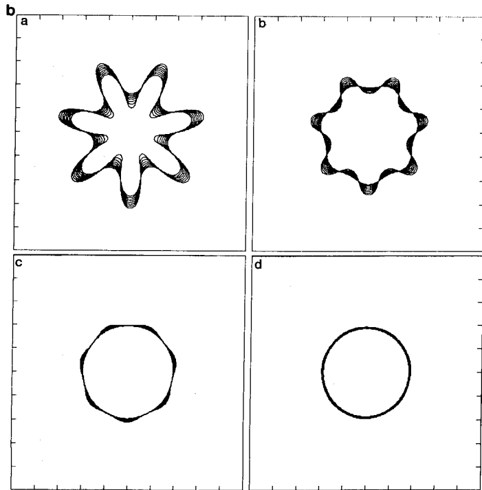
FIG. 4b. Star-shaped curve collapsing under curvature (Continued) F(K) = -K : (a) T = 0.0, 0.5 (0.005); (b) T = 0.5, 1.0 (0.005); (c) T = 1.0, 1.5 (0.005); (d) T = 1.5, 2.0 (0.005).
