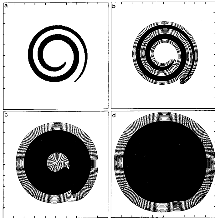
FIG. 6. Burning spiral: merging and breaking F(K) = 1 - \varepsilon K , \varepsilon = 0.01 : (a) T = 0.0 (initial curve); (b) T = 0.00, 0.03 (0.01); (c) T = 0.04, 0.12 (0.01); (d) T = 0.13, 0.22 (0.01).
