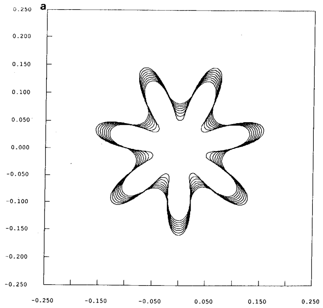
FIG. 4a. Star-shaped curve collapsing under curvature (Beginning): F(K) = -K , T = 0.0, 0.5 (0.005).
