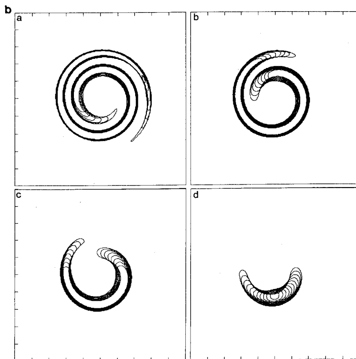
FIG. 5b. Wound spiral collapsing under curvature (Complete history) F(K) = -K : (a) T = 0.0, 0.065 (0.01); (b) T = 0.065, 0.130 (0.01); (c) T = 0.130, 0.195 (0.01); (d) T = 0.195, 0.295 (0.01).
