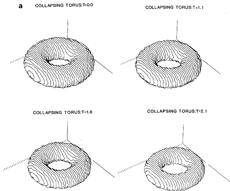
FIG. 14a. Collapse of torus under mean curvature (Beginning): F(K) = -K , T = 0.0, 1.1, 1.6, 2.1 .
