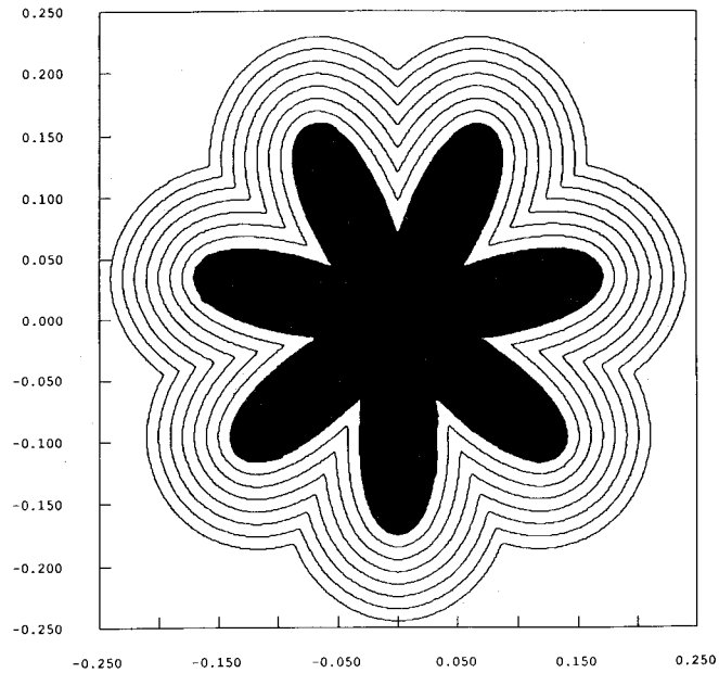
FIG. 3. Star-shaped front burning out: F(K) = 1 , T = 0.0, 0.7 (0.01) .
