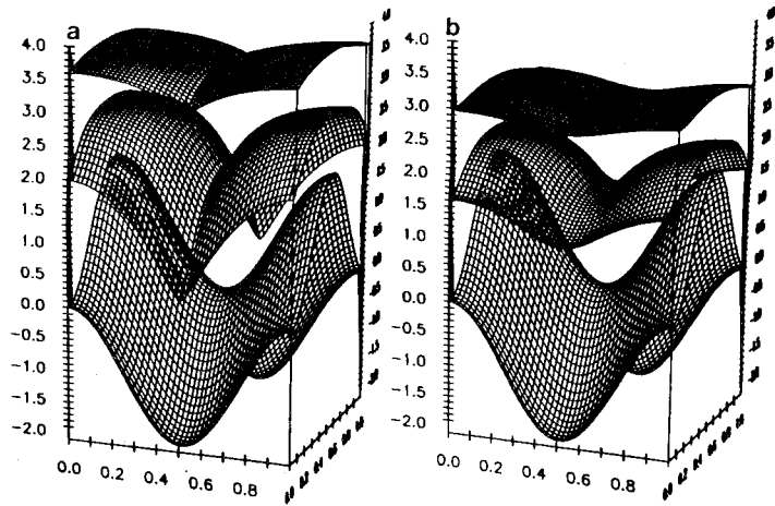
FIG. 9. Propagating surface: F(K) = 1 - \epsilon K , mean curvature: (a) F(K) = 1 , surface at T = 0.0, 0.3, 0.6 ; (b) F(K) = 1 - \epsilon K , \epsilon = 0.1 , surface at T = 0.0, 0.3, 0.6 .
