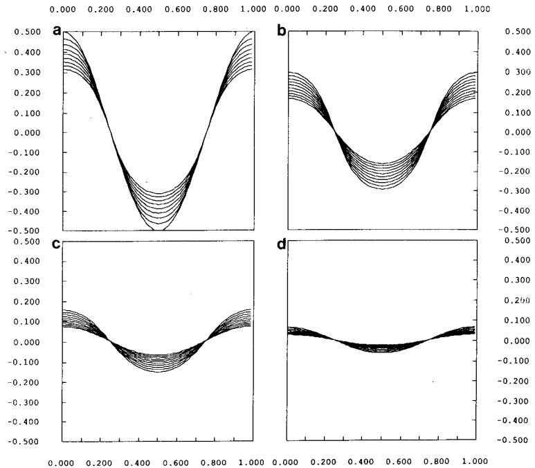
FIG. 2. Propagating initial sine curve: F(K) = -K . Motion under curvature: Plots of \psi vs. x . (a) F(K) = -K , Plots at t = 0.0, 0.5 (0.05); (b) F(K) = -K , Plots at T = 0.5, 1.0 (0.05); (c) F(K) = -K , Plots at T = 1.0, 1.5 (0.05); (d) F(K) = -K , Plots at T = 1.5, 2.0 (0.05). \psi(x, 0) = \sin(2\pi x) .
