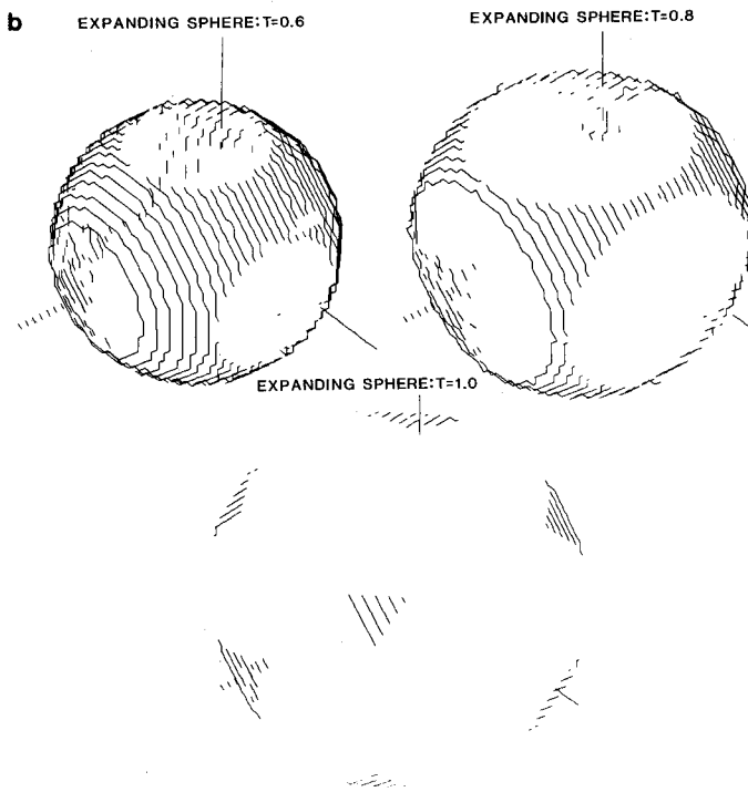
FIG 11b. Sphere burning outwards (Continued): F(K) = 1 , surface at T = 0.6, 0.8, 1.0 .
