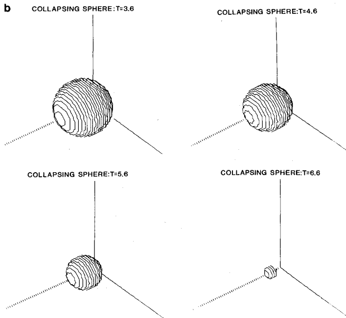
FIG. 13b. Sphere collapsing under mean curvature (Continued): F(K) = -K , surface at T = 3.6, 4.6, 5.6, 6.6 .
